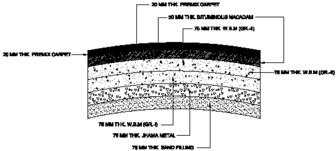
CROSS SECTIONAL ELEVATION OF BITUMINOUS PAVEMENT (APPROACH ROAD)
