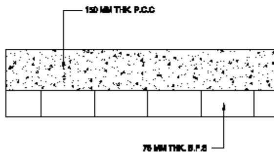
CROSS SECTIONAL ELEVATION OF CONCRETE PAVEMENT (APPROACH ROAD)
