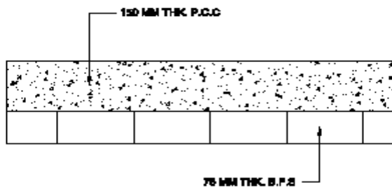
CROSS SECTIONAL ELEVATION OF CONCRETE PAVEMENT (APPROACH ROAD)
