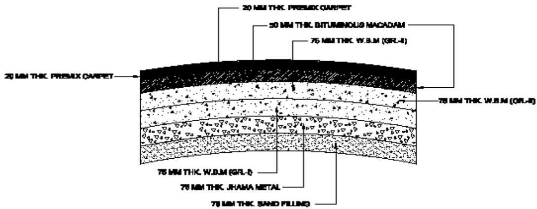
CROSS SECTIONAL ELEVATION OF BITUMINOUS PAVEMENT (APPROACH ROAD)
