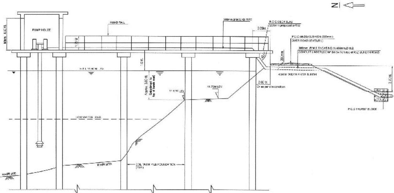
3.00 MTR. WIDE R.C.C PIPE CARRYING BRIDGE
