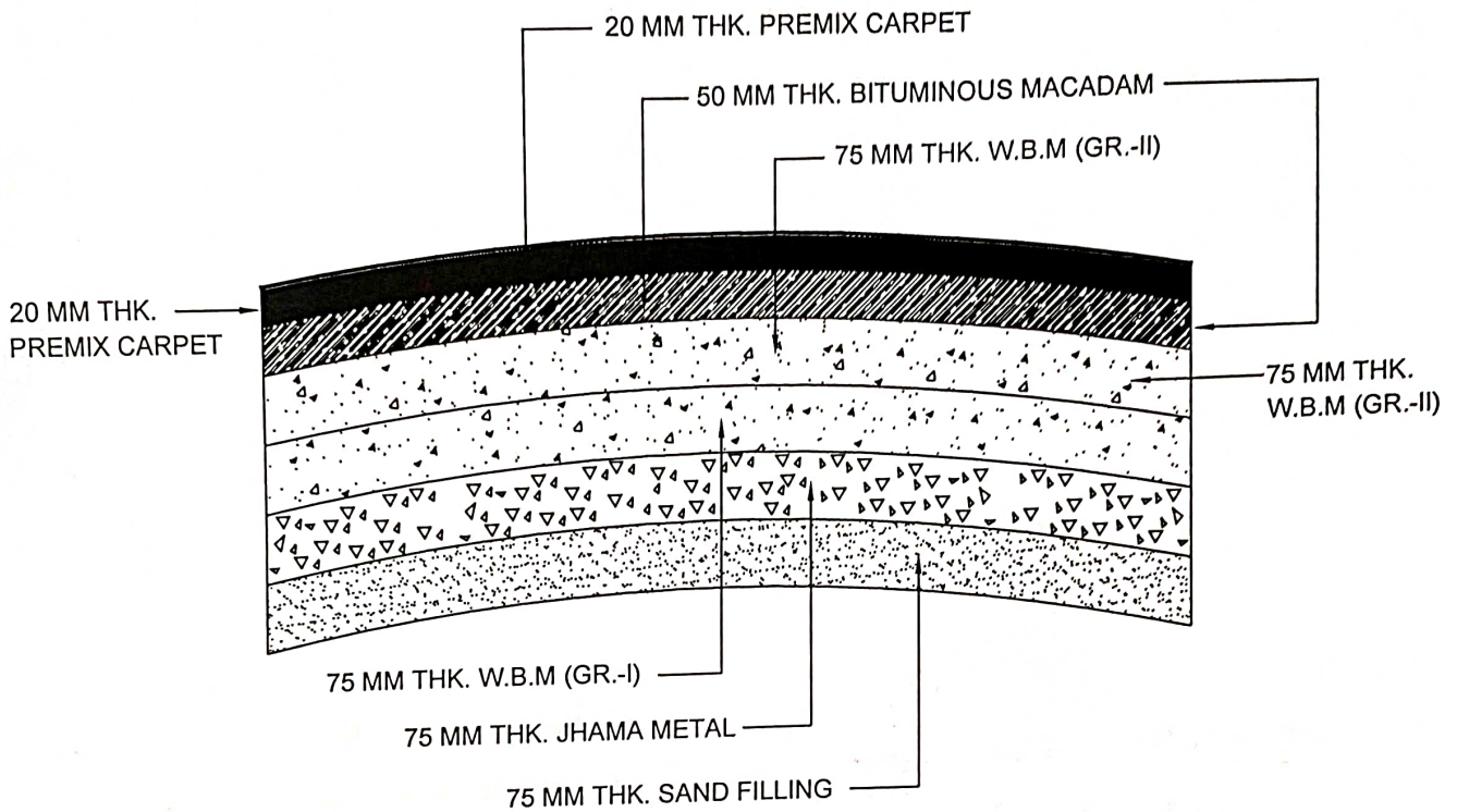
CROSS SECTIONAL ELEVATION OF BITUMINOUS PAVEMENT (APPROACH ROAD)
