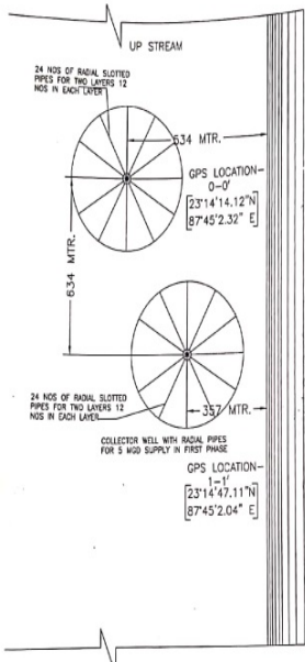
KEY PLAN FOR COLLECTOR WELLS
