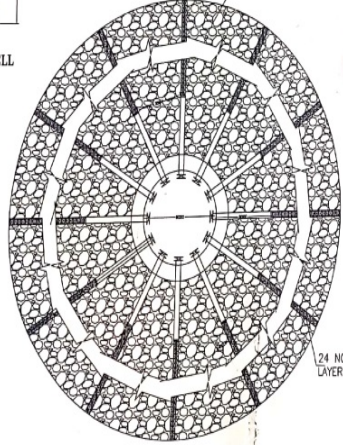
PLAN SHOWING BOULDER SAUSAGE WORK AND REDIAL COLLECTOR WELL
