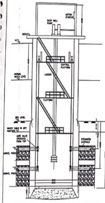
SECTION OF COLLECTING WELL
